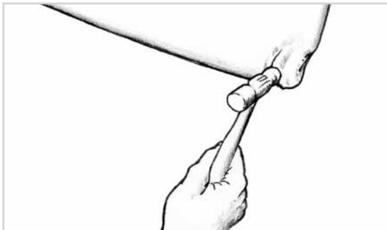
Figure 8-2 Use a ball-peen hammer, with repeated light taps to work the lead bulge back to its original shape.
