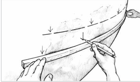
Figure 14-9 Use a long batten to locate the high and low areas and judge the amount of fairing compound required
