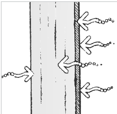
Figure 9-2 Polyester resins and gelcoats allow water molecules to migrate into the laminate and dissolve soluble materials within the laminate.
